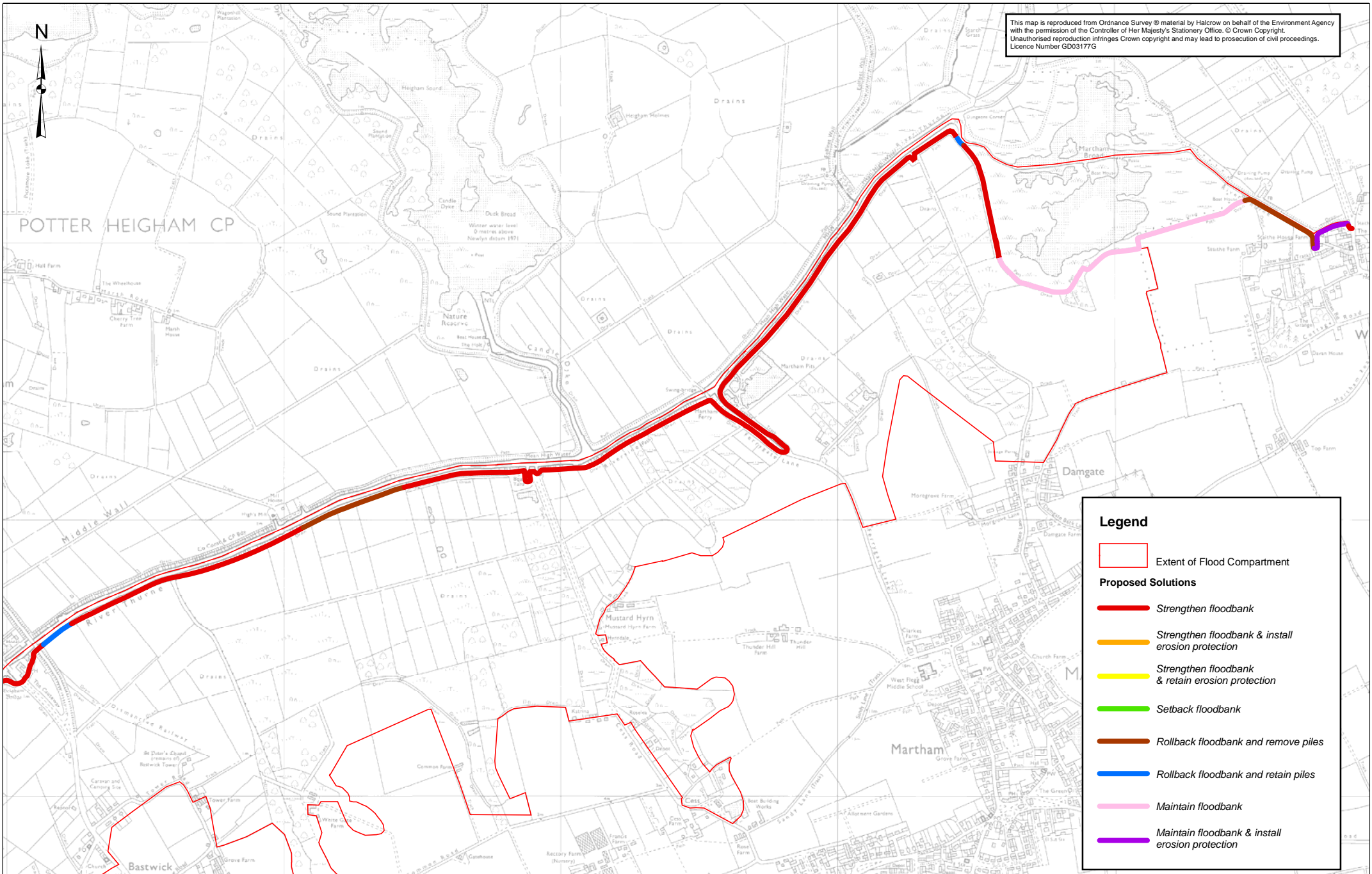
Flood Defence Proposals for Thurne to West Somerton (Compartment Number 07) Updated for Broads Authority Walkover 11 January 2007
